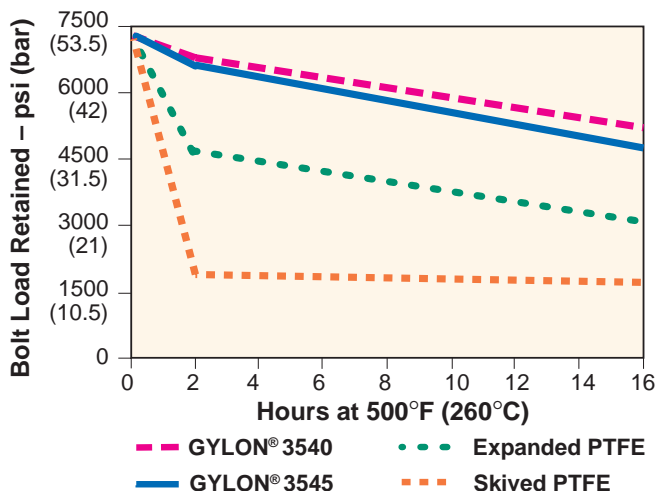
Figure 5: DIN 52913 Gasket Bolt Load vs. Time
